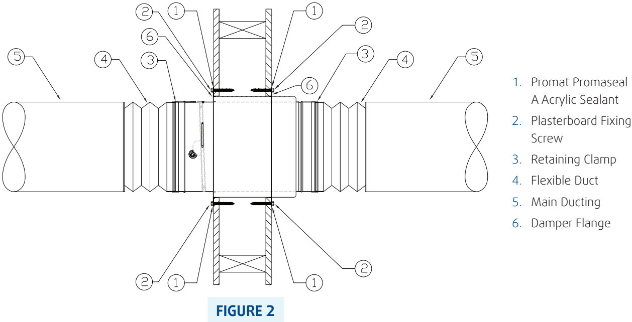
Single Layer 16mm Fire Rated Plasterboard FRL: -/90/- Installation
