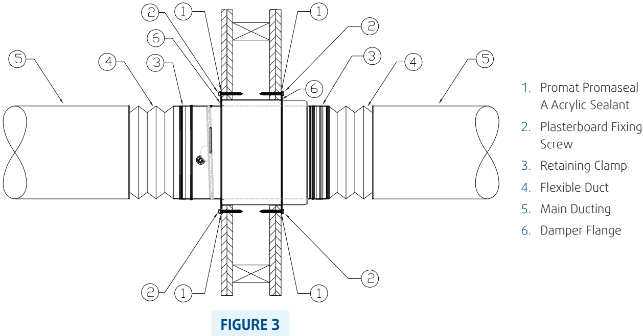
Double Layer 13mm Fire Rated Plasterboard FRL: -/120/- Installation
