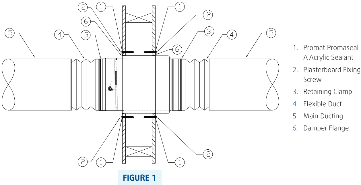
Single Layer 13mm Fire Rated Plasterboard FRL: -/60/- Installation
